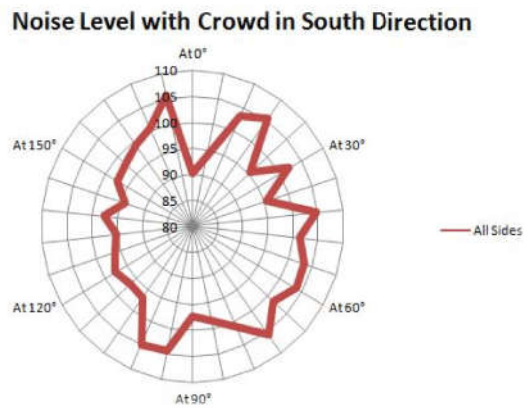
Fig. 14. Surround Noise Level in N-S direction
