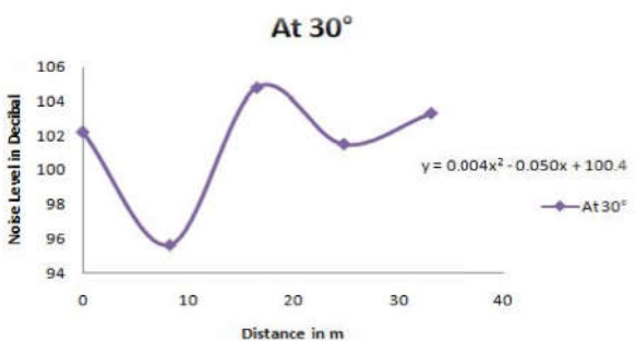
Fig. 10 Noise Level in N-S direction at 30°
