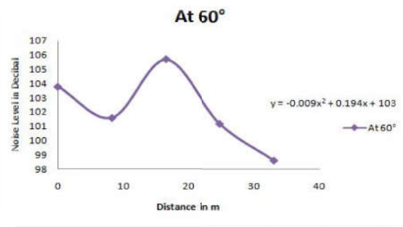
Fig. 11. Noise Level in N-S direction at 60°
