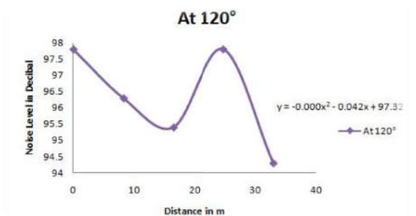
Fig. 13 Noise Level in N-S direction at 120°
