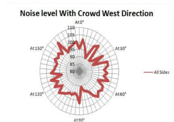
Fig. 8 Surround Noise Level in E-W direction
