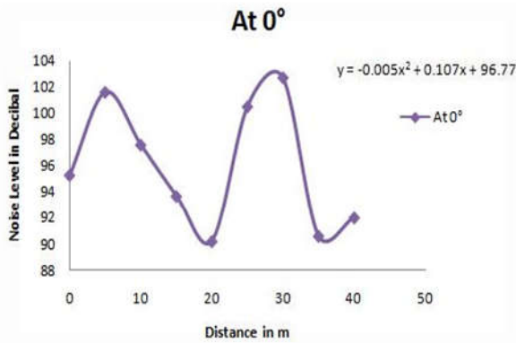
Fig. 3. Noise Level in E-W direction at 0°
