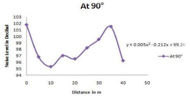
Fig. 6 Noise Level in E-W direction at 90°
