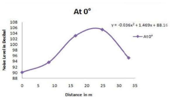
Fig. 9 Noise Level in N-S direction at 0°
