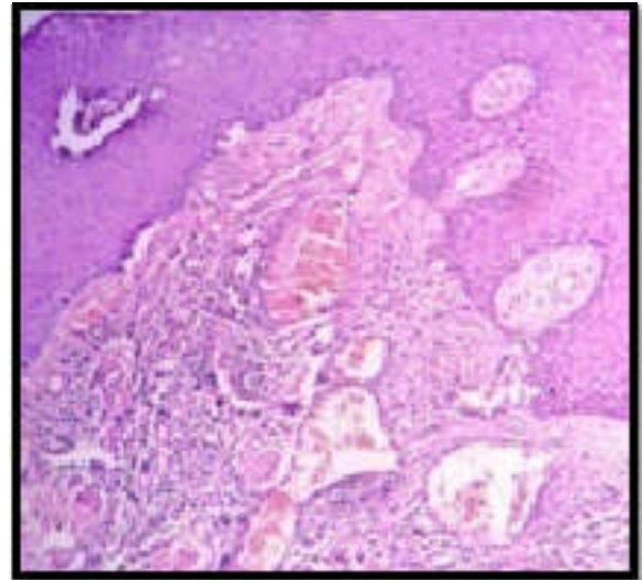
Fig. 5. Histopathological photograph suggested to be pyogenic granuloma
