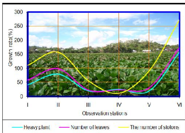
Figure 2. Growth Rate Comparison Chart E. crassipes (Source: Murdianto et al. , 2007)
