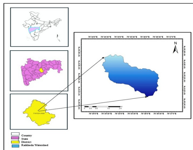
Fig. 1 Location Map of Raikheda watershed
