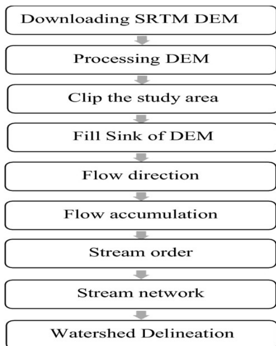
Fig. 2. Steps in Watershed Delineation
