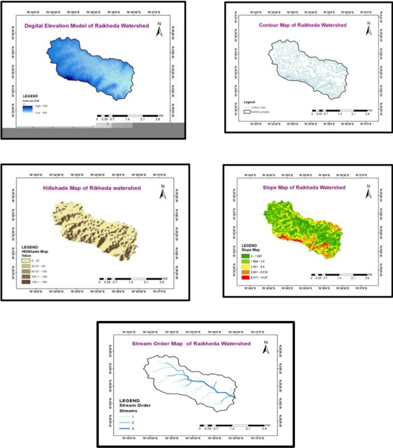
Fig. 3. Various maps of Raikheda watershed
