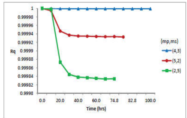
Fig. 2. Effect of (mp, ms) on query reliability (Rq).
