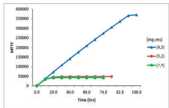
Fig. 3. Effect of (mp,ms) on MTTF
