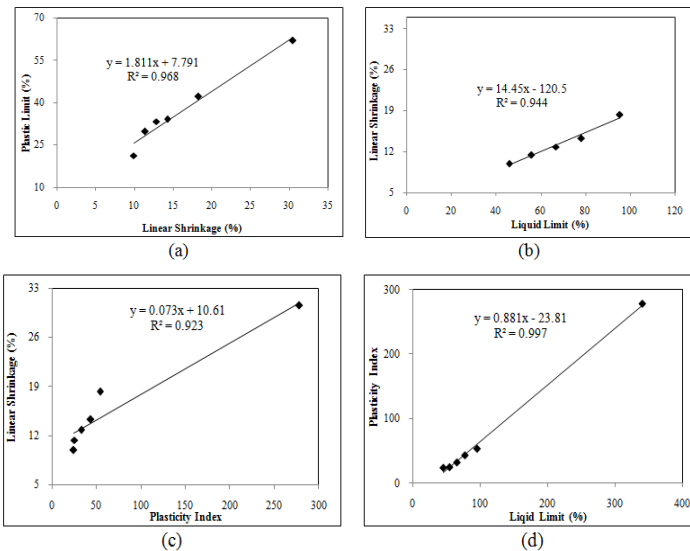
Fig. 4. Relationship among different geo-engineering properties of the samples- (a) linear shrinkage and plastic limit, (b) liquid limit and linear shrinkage, (c) plasticity index and linear shrinkage and (d) liquid limit and plasticity index
