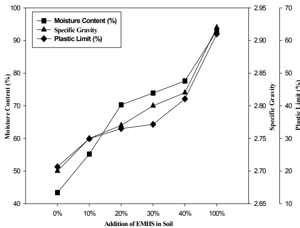
Fig. 1. Moisture content, specific gravity and plastic limit of EMHS and EMHS amended soil
