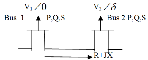
Fig. Two-bus power system model
