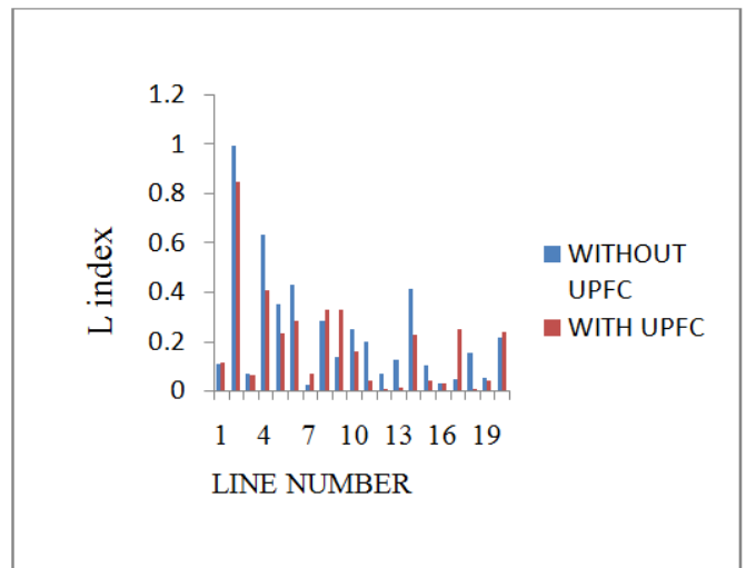
Fig. Comparison of L index
