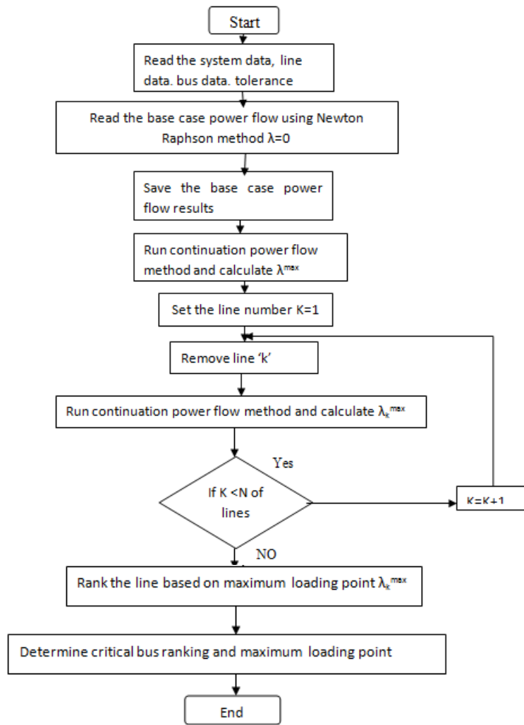
Fig.2. Flow chart for optimal power flow
