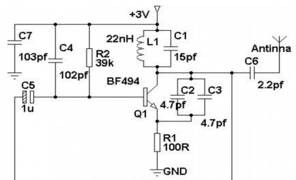
Fig.1 Connection circuit
