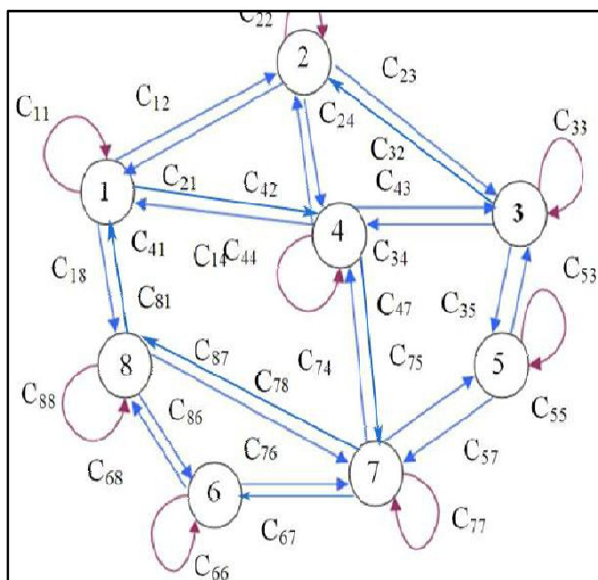
Figure 1. Cluster communication
