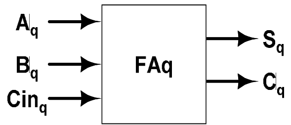
Figure 2. Proposed quaternary full adder
